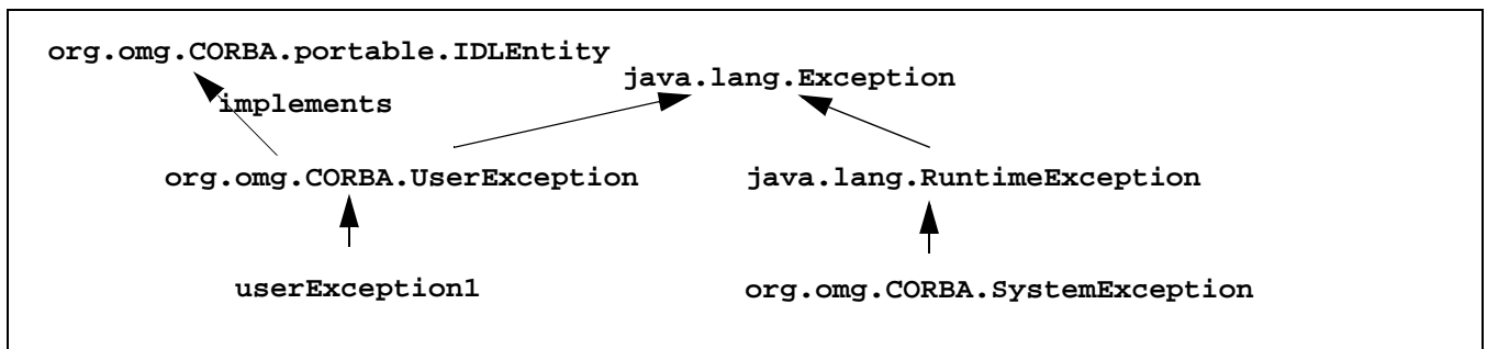
Figure 2-1 Inheritance of Java Exception Classes
