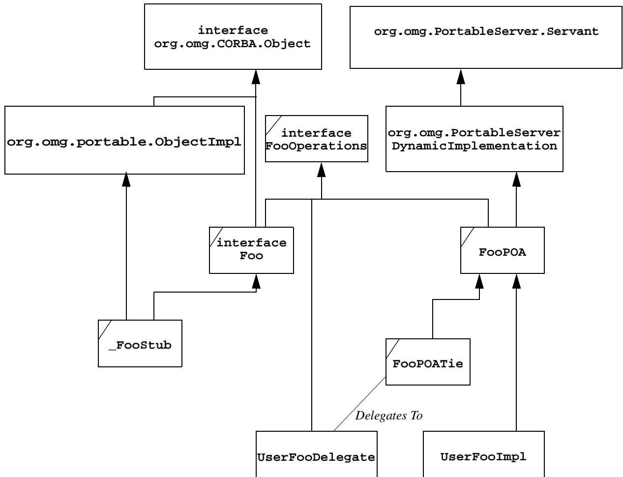
Figure 2-2 Class hierarchy for portable Java stubs and skeletons
