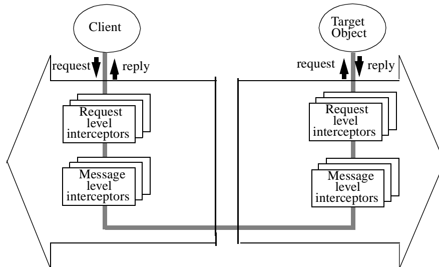
Figure 21-1 Interceptors Called During Invocation Path
