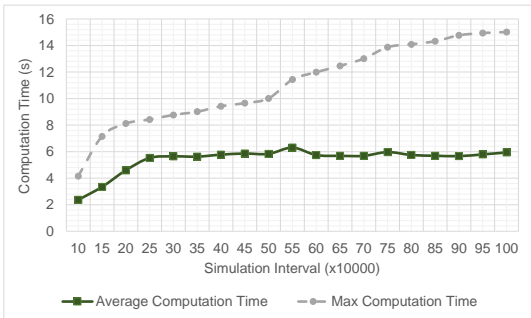
Figure 4: Computation time of the simulator
