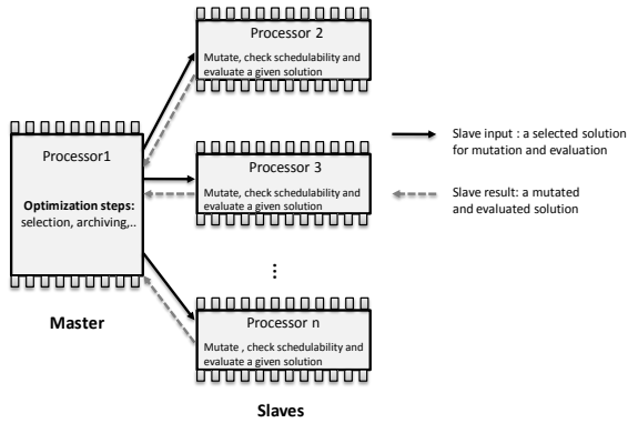
Fig. 3: Master-Slave Model
