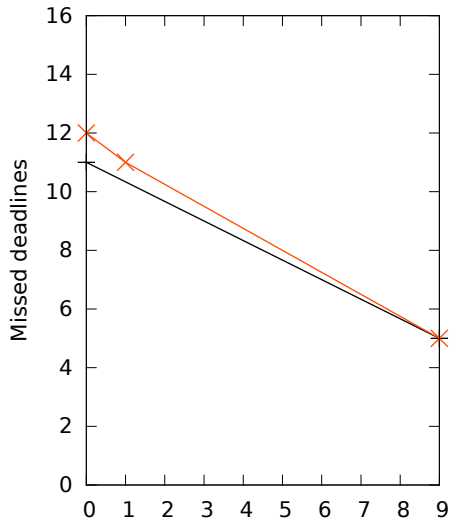
Integrity - Biba rules violations (mix-grain)
