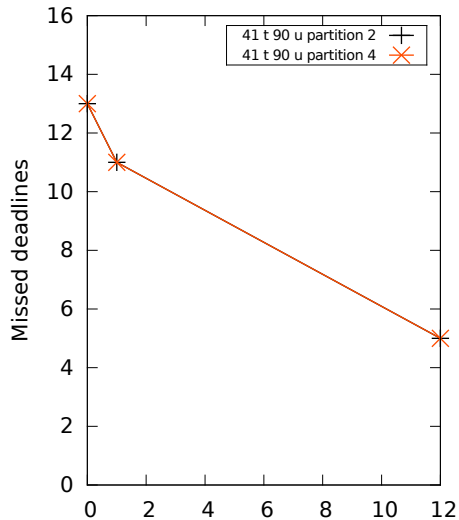
Confidentiality - BLP rules violations (mix-grain)
